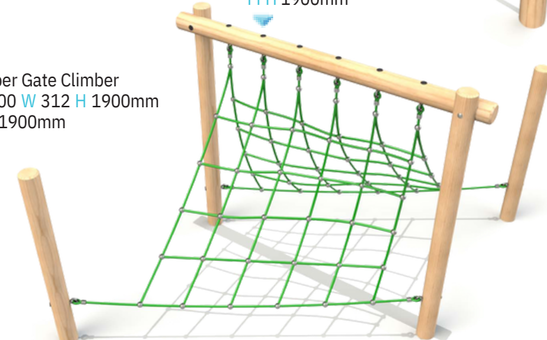
Twist Net L 3200 W 2295 H 1900mm FFH 1900mm
