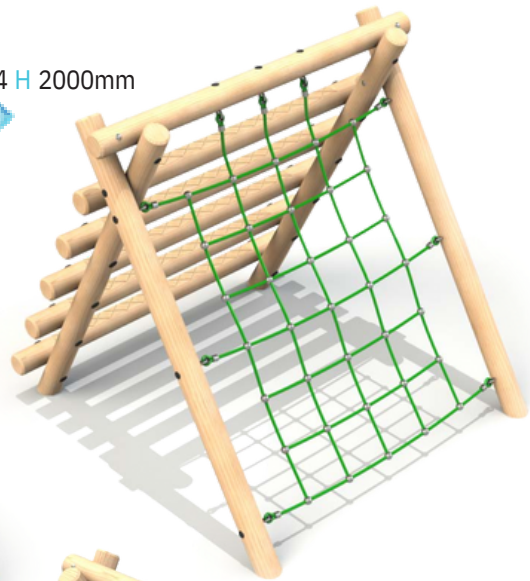
A-Frame Low L 1974 W 1600 H 1500mm FFH 1500mm
