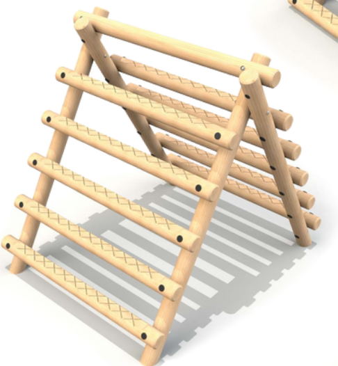
Log Climber High L 2093 W 1849 H 2000mm FFH 2000mm
